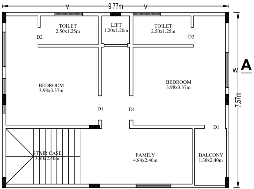
PROPOSED TYPICAL 1 & 2 FLOOR PLAN
